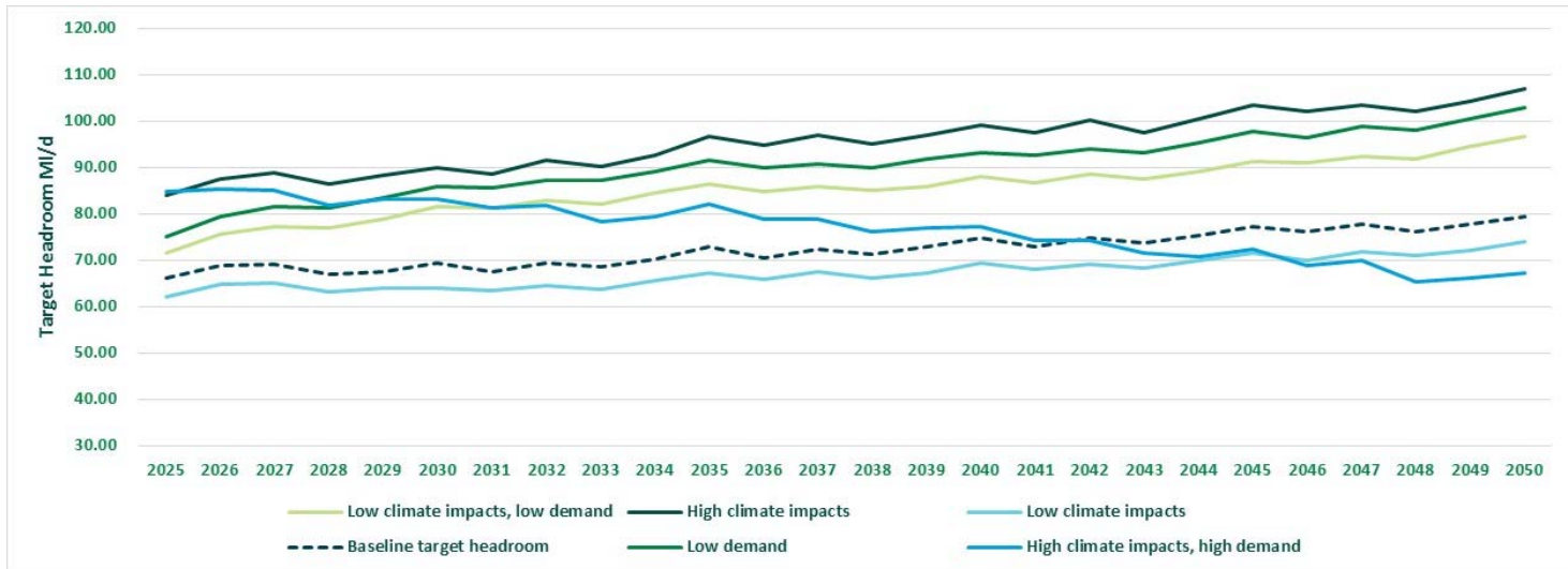
Figure 13 Target headroom profiles for adaptive planning - Strategic Resource Zone
