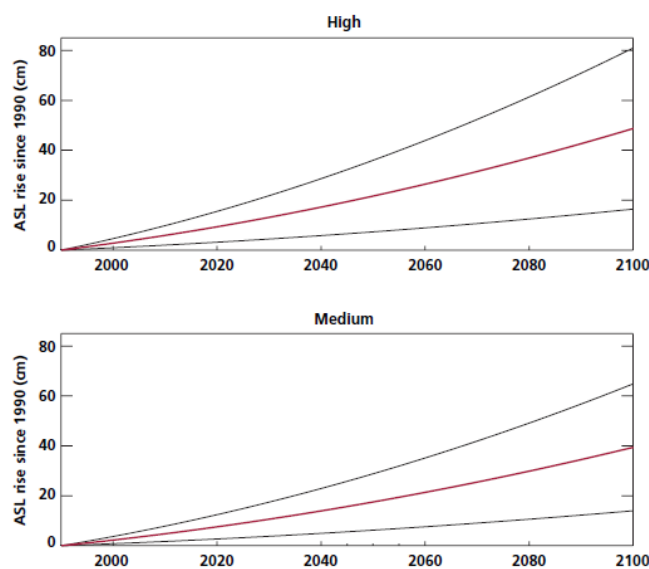
Figure 3.4: Estimated UK absolute sea level (ASL) rise time series for the 21st century (representing the average for masked region shown in Figure 3.3). Central estimates (thick lines) for each of three scenarios (low, medium and high emissions) shown together with range given by 5th and 95th percentiles (thin lines).
