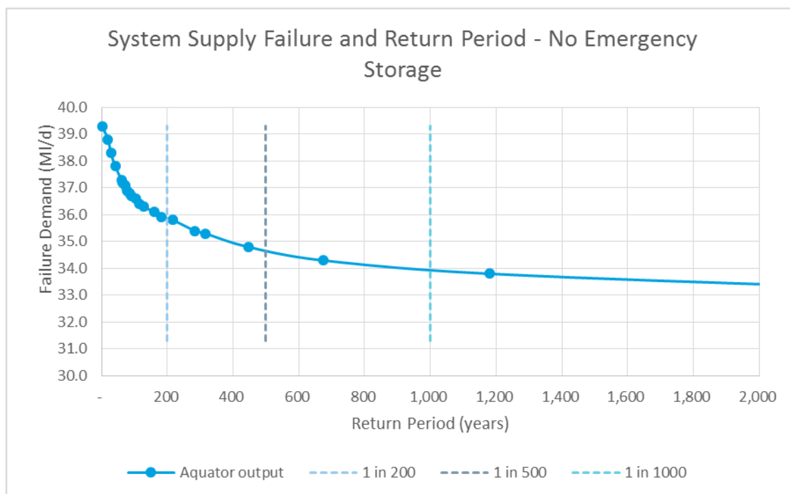
Figure 14 System supply failure and return period in the Carlisle Resource Zone
