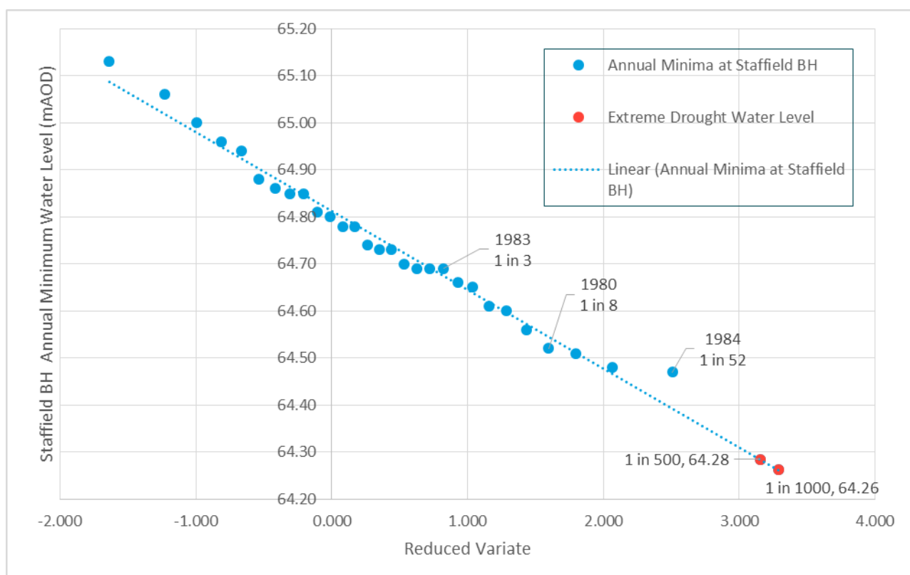
Figure 15 Extreme value plot for groundwater level in North Eden Resource Zone
