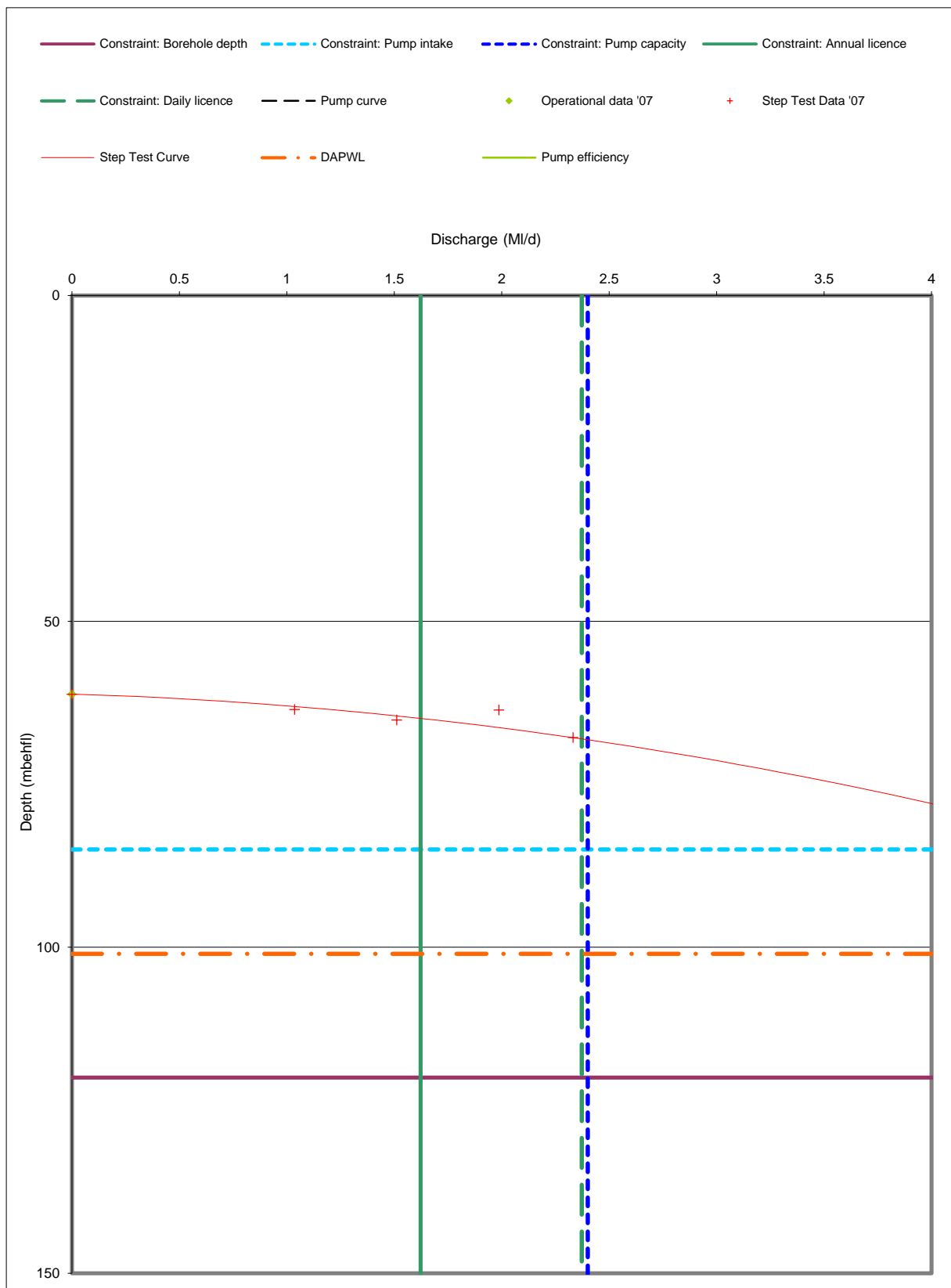
Figure 24 Source reliable output diagram for a groundwater source in the North Eden Resource Zone
