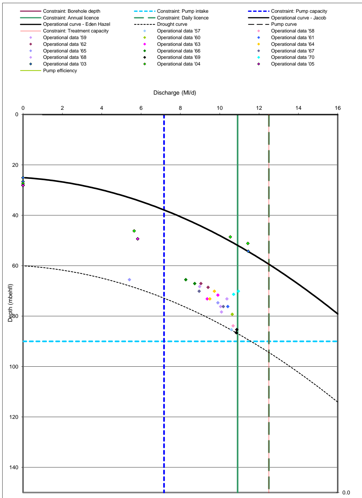
Figure 23 Source reliable output diagram for a groundwater source in the Strategic Resource Zone
