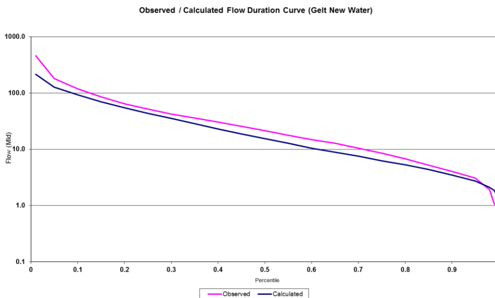
Figure 19 Flow duration curve from the River Gelt (New Water) rainfall-runoff model, using parameters from the 2012 work
