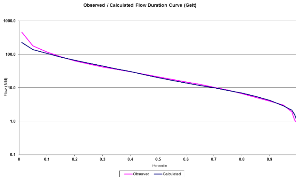
Figure 21 Flow duration curve from the River Gelt (New Water) rainfall-runoff model, using parameters from the 2016 work
