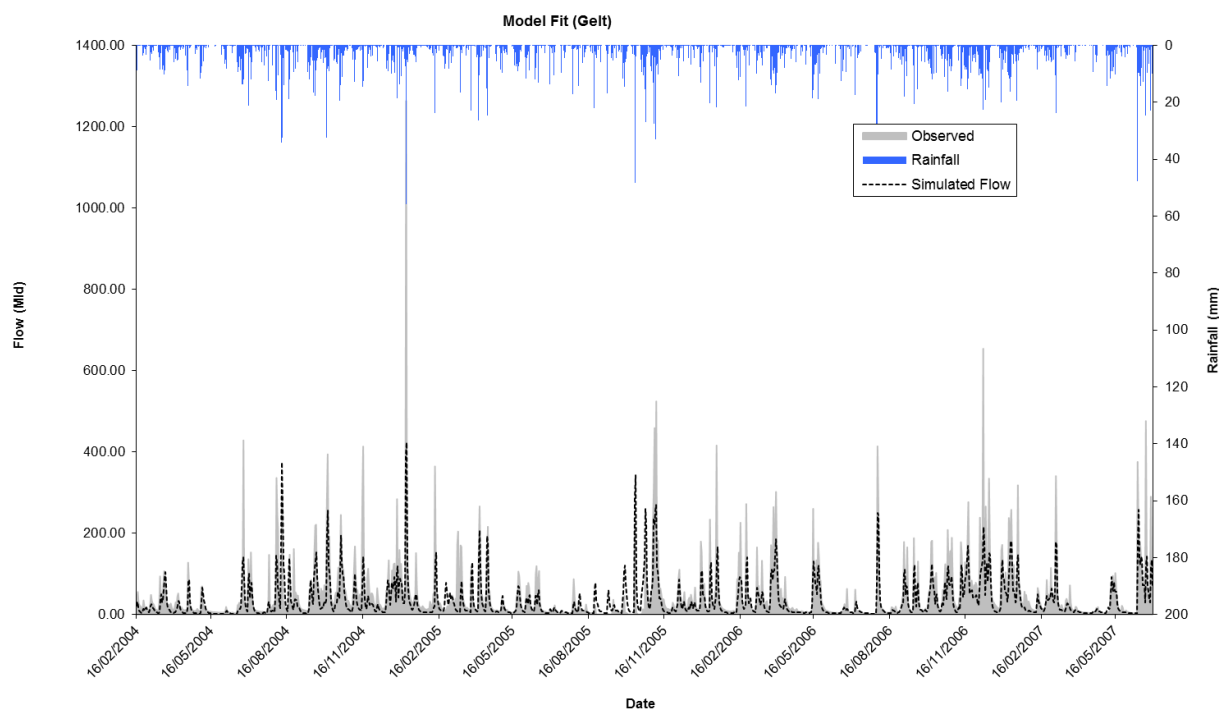
Figure 18 River Gelt (New Water) rainfall-runoff model fit, using parameters from the 2012 work
