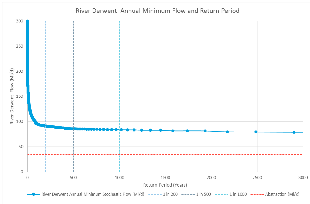
Figure 16 Return Period for Annual Minimum Flow in the River Derwent (Barepot Resource Zone)
