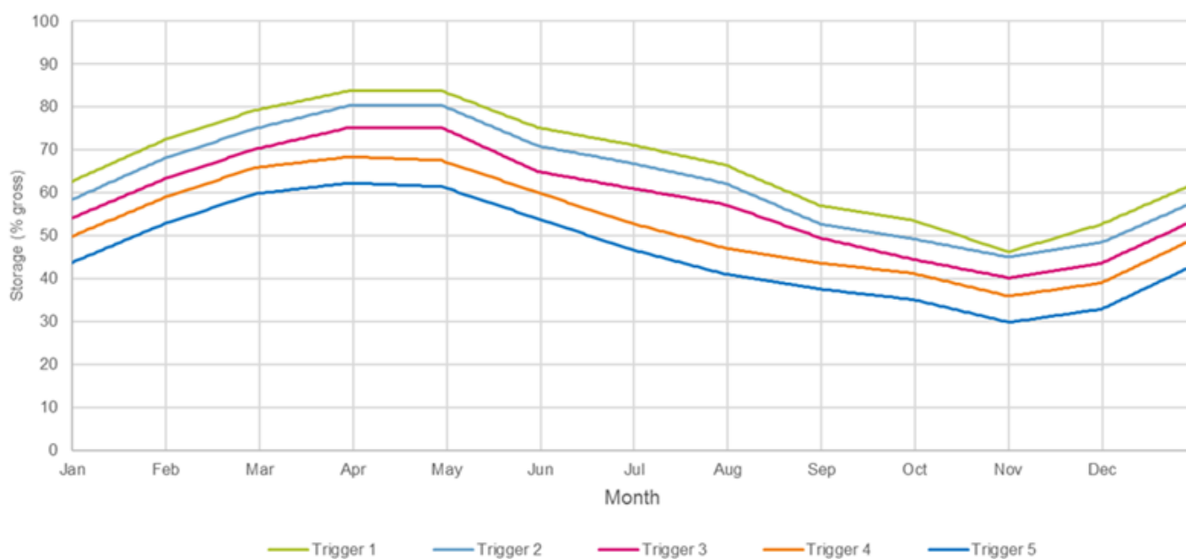
Figure 22 Haweswater drought triggers including hypothetical trigger 5 for future drought permits and orders implementation
