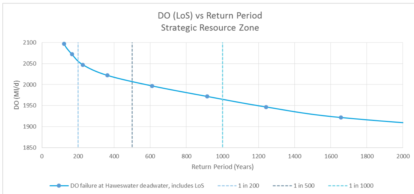
Figure 13 Strategic Resource Zone deployable output (with level of service) and return period
