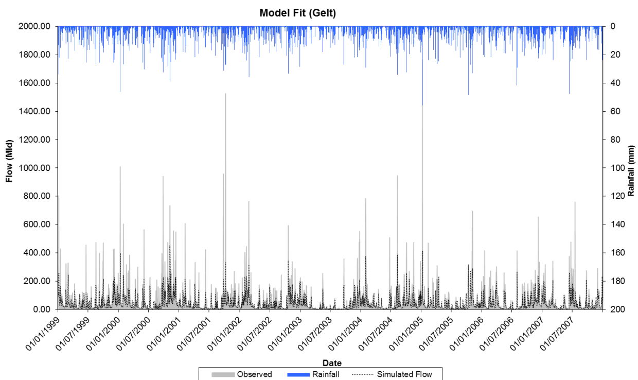
Figure 20 River Gelt (New Water) rainfall-runoff model fit, using parameters from the 2016 work
