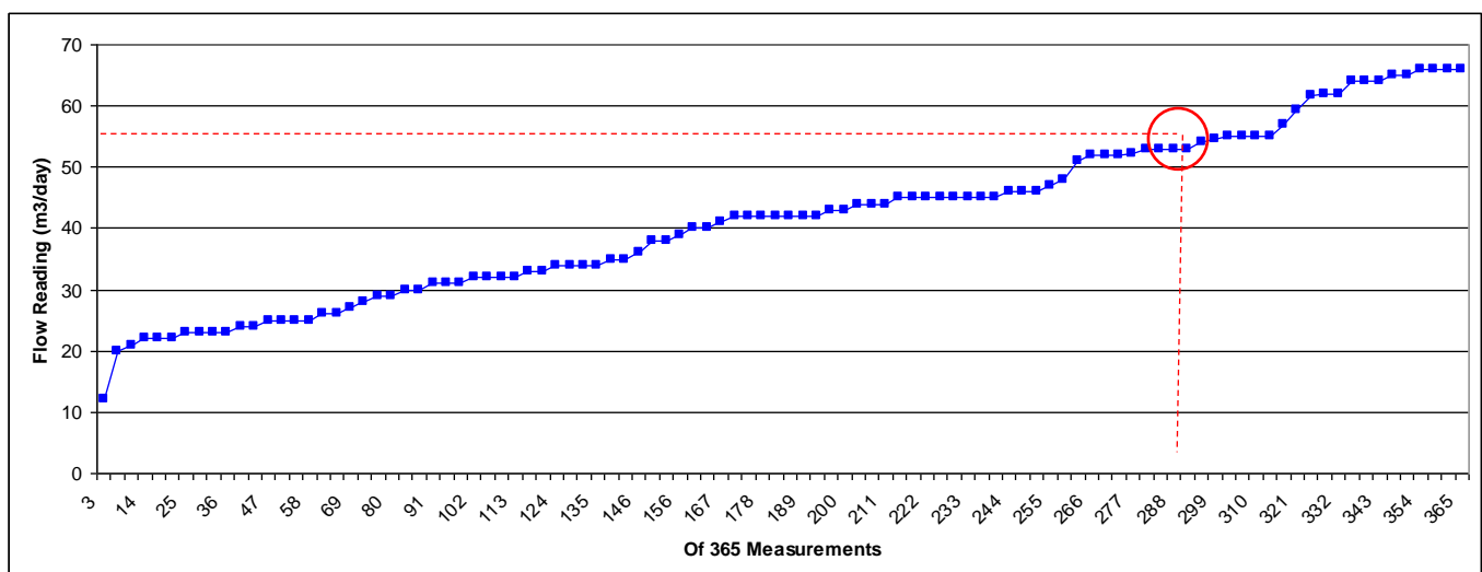
Figure 5 Q80 Calculation for wastewater treatment works using total daily volumes. (Q80 is the 292nd total daily volume when ranked)
