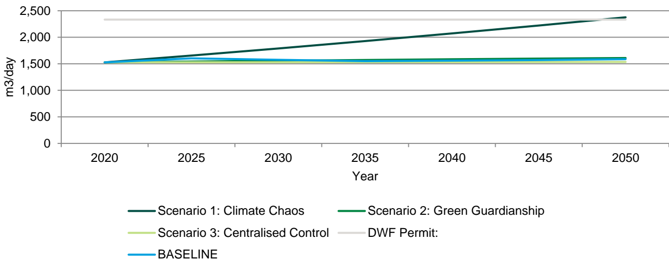
Figure 13 Applying different assumptions to elements of demand to forecast future dry weather flow
